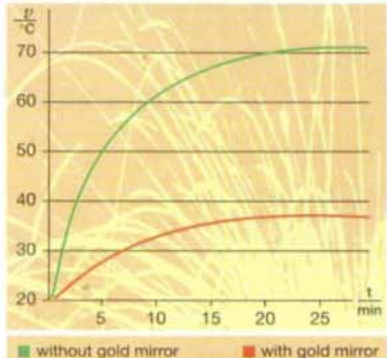
Heating of ATHERMAL shade 11 A 1 DIN, with and without gold mirror coating (measurement conditions: welding with 6 mm electrodes, current intensity 350 Amperes working distance 40 cm)
